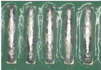
洗浄前 Before cleaning
